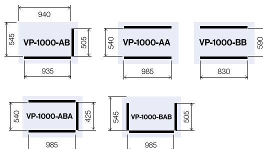
VP-1000 High lid AB, AA, BB, ABA, BAB, AB, HIGH. BUSCH pump 100m³/h.
