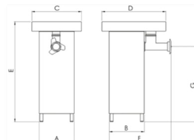
TOP-114. Production \pm 1.000 kg/h. Motor Power 5.5HP.
