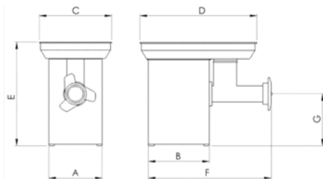
SUPERSTAR. Production \pm 800 kg/h. Motor Power 3.5HP.
