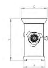
P-22. Production \pm 300 kg/h. Motor Power 1.5HP. P-32. Production \pm 425 kg/h. Motor Power 2.5HP.
